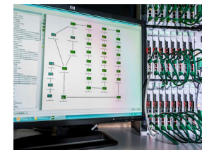
Networked systems
